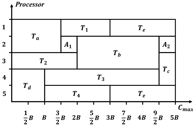
Fig. 3. A feasible schedule with C_{max} = 5B for the clockwise direction of a five-node ring with shortest path routing.
